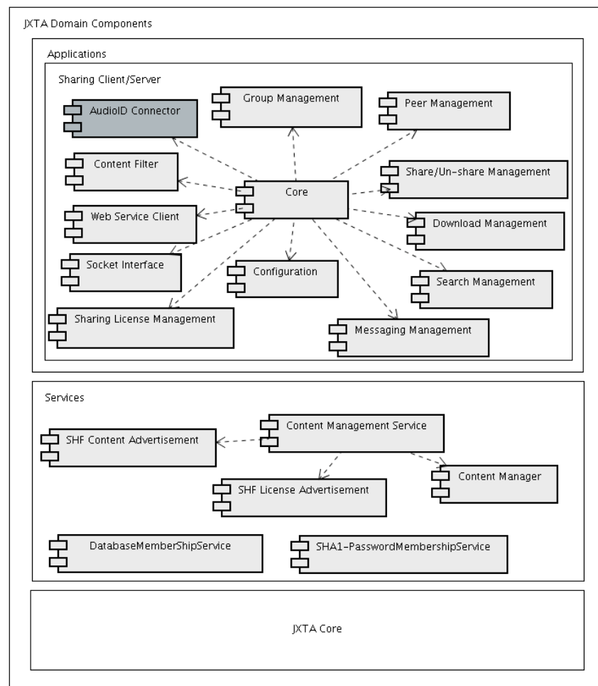
Figure 1: Developed components within the JXTA architecture model
